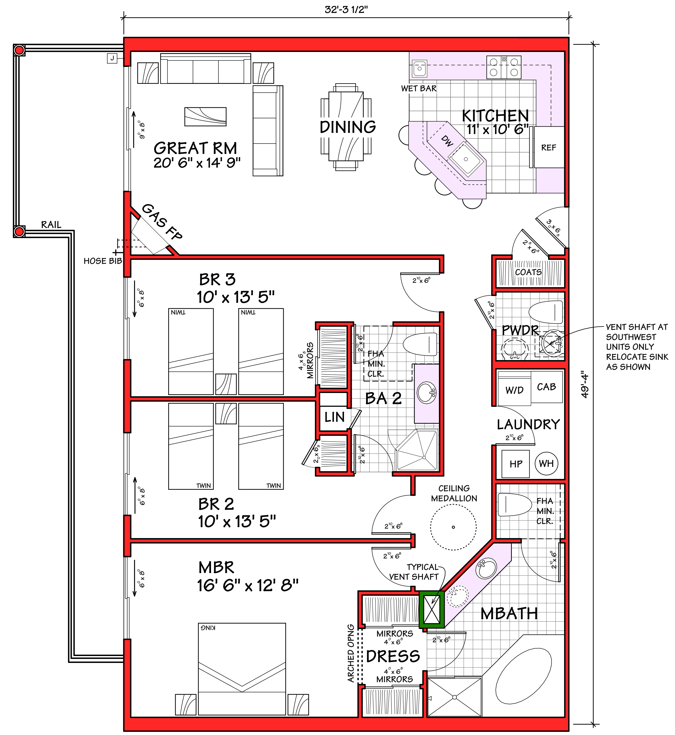
UNIT 2 - 3BR FLOOR PLAN AREA: 1593 SQ FT BALCONY AREA: 235 SQ FT
