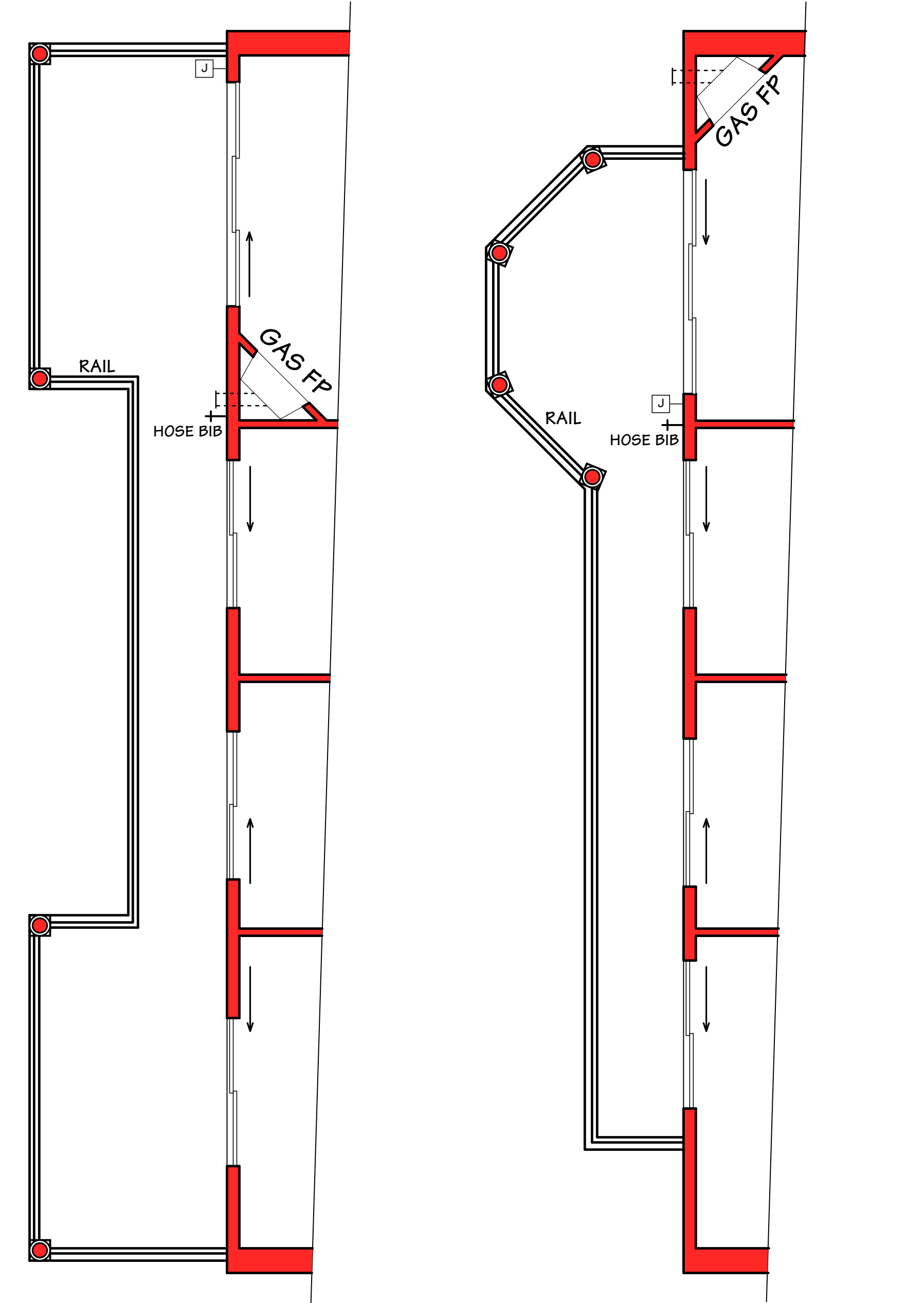
UNIT 2 - ALTERNATE BALCONIES BALCONY AREA: 310 SQ FT BALCONY AREA: 200 SQ FT
